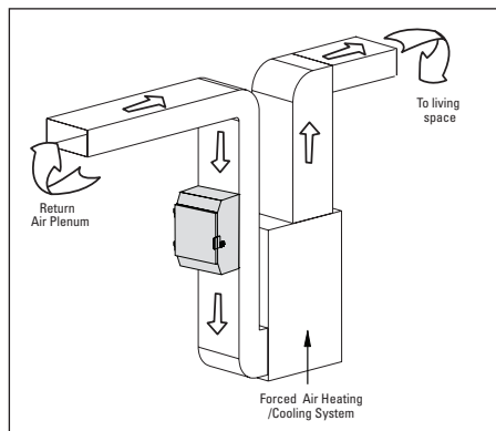
HEPA Mounted on Duct
